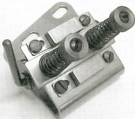
Tensor
